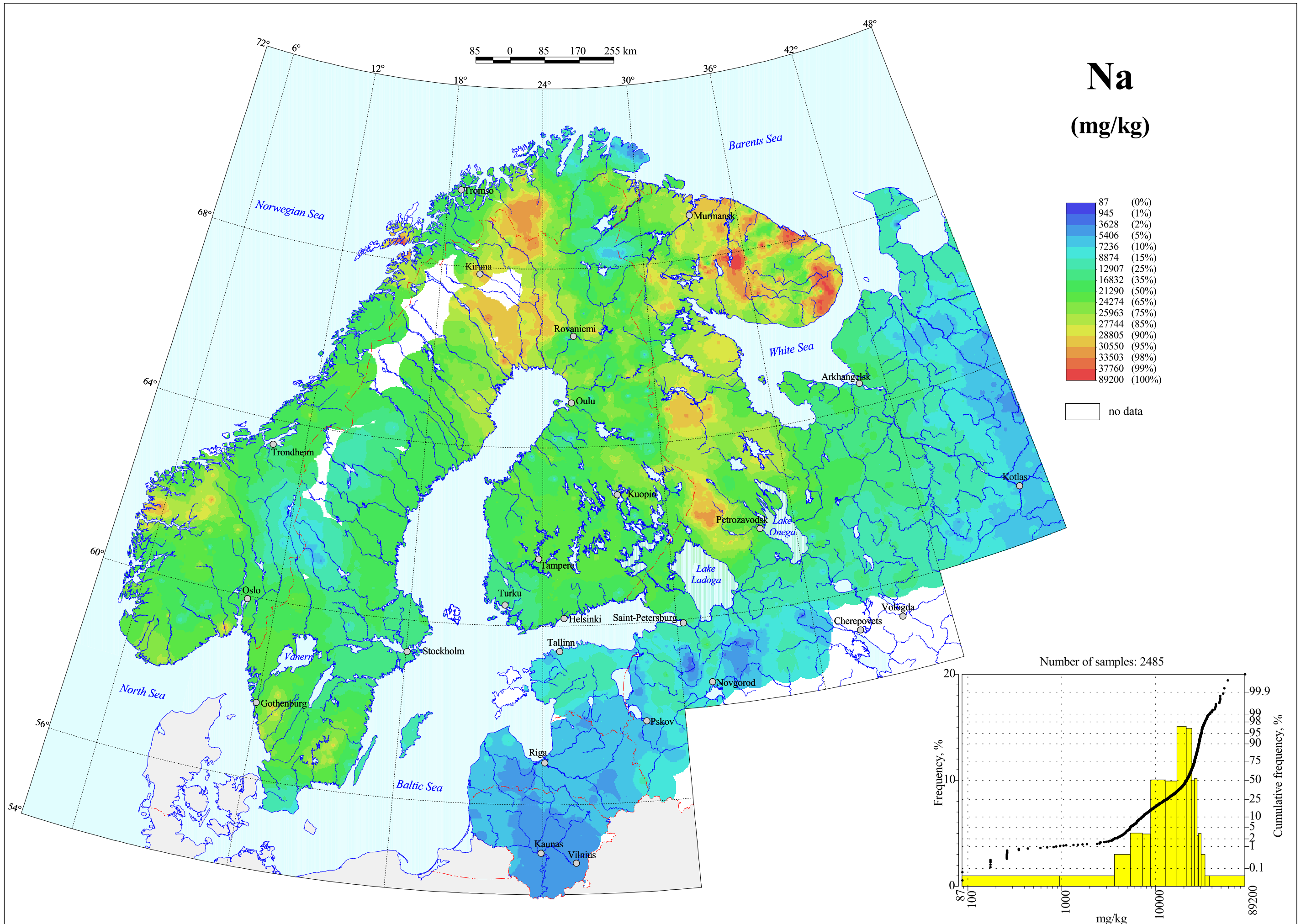
Sodium in C-horizon, Grain Size <2 mm, Total Content
